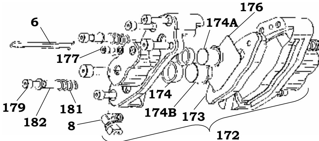
Billet 4 spot Caliper VEN99
