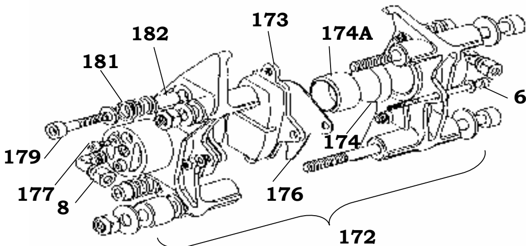
Cast 2 spot Caliper VEN91
