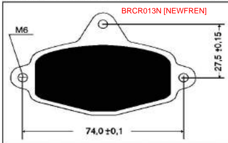
Figure 6 [74 mm Centres 6mm Threaded Holes] 14mm Thick
