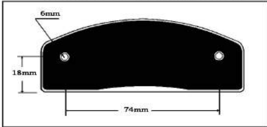
Figure 5 [ 56mm Centres 6mm Threaded Holes ] 17mm Thick Figure 5A [ 65mm Centres 6mm Threaded Holes ] 17mm Thick Figure 5B [ 74mm Centres 6mm Threaded Holes ] 17mm Thick
