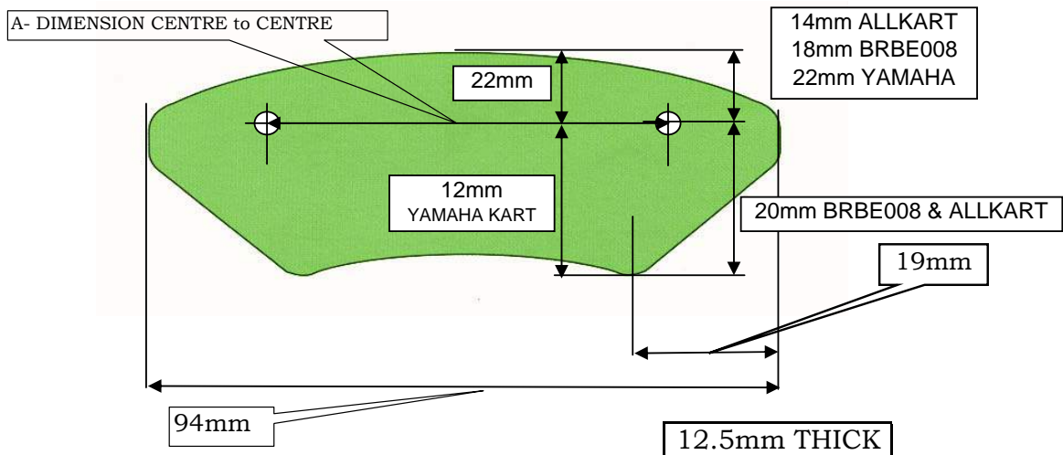
UNIVERSAL BRAKE PADS FITS MANY BRANDS OF KARTS
