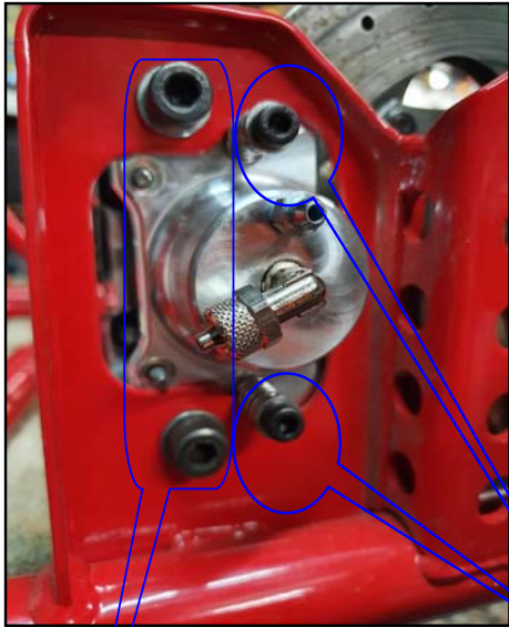
DENT 2 SPOT CALIPER FITTED TECNO KART
